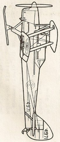
DH-82C TIGER MOTH, Royal Canadian Air Force, 1943. No. 19 Elementary Flying Training School
